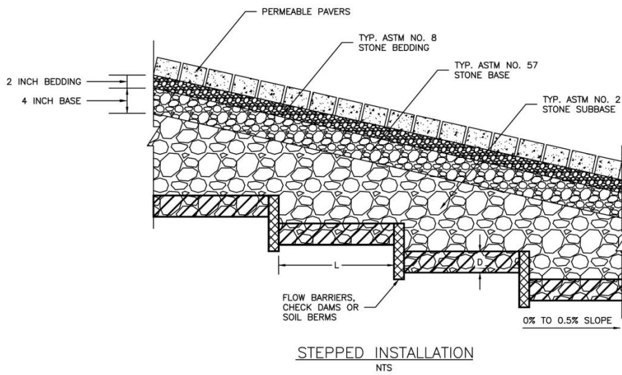
Figure 5.4-11. Stepped Installation Section
