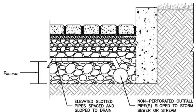
Figure 5.4-5. PICP Facility with Elevated Drain
