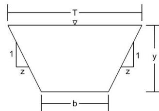
Figure 5.6-3. Trapezoid Dimensions
