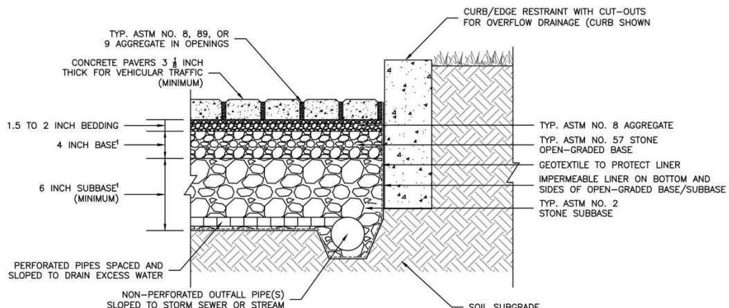
NO INFILTRATION NTS
