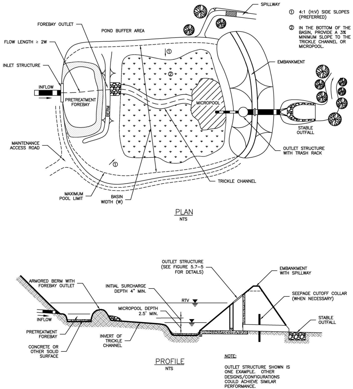
Figure 5.7-7. Extended Detention Basin Plan View and Typical Section Source: Adapted from UDFCD (44)
