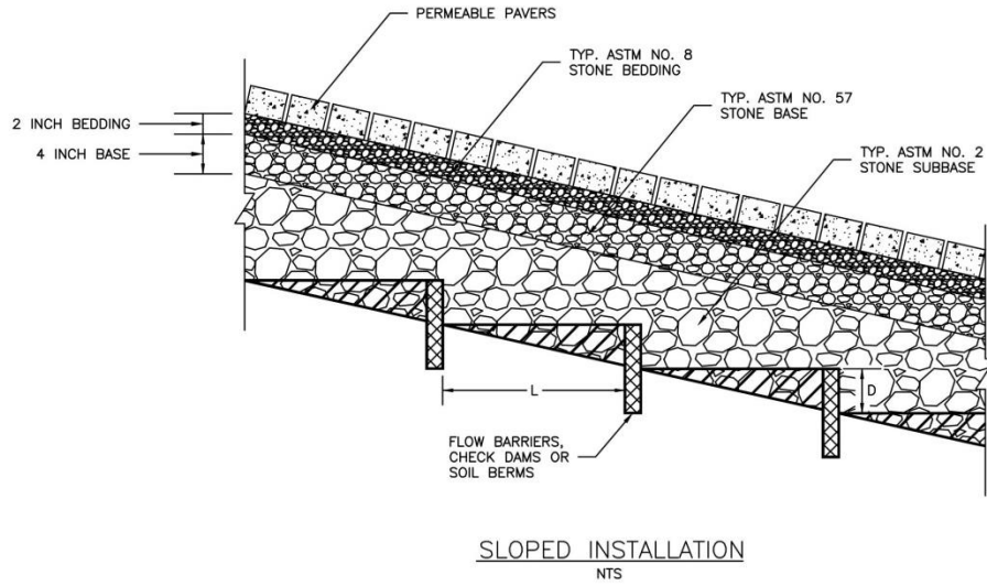
Figure 5.4-10. Sloped Installation Section
