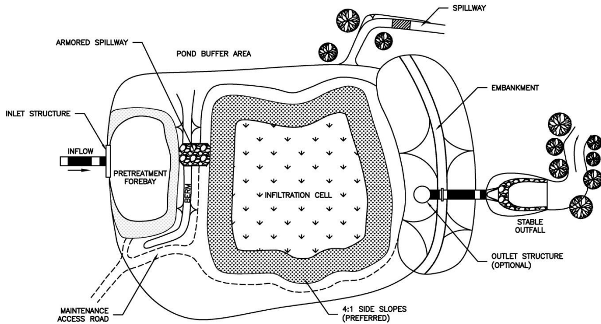
PLAN NTS
