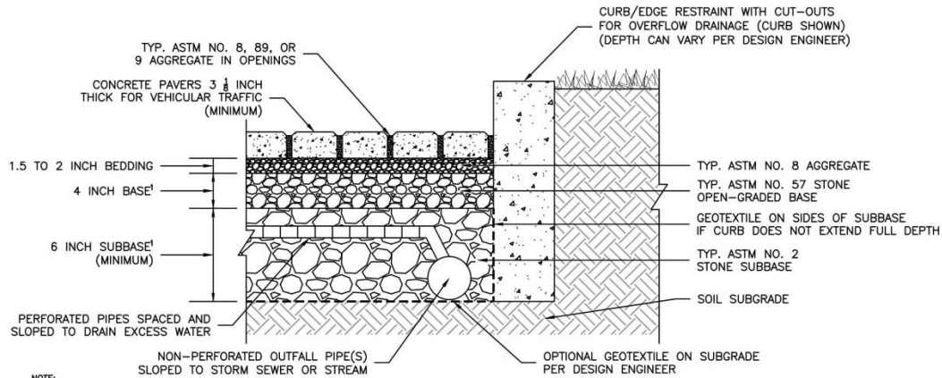
PARTIAL INFILTRATION NTS
