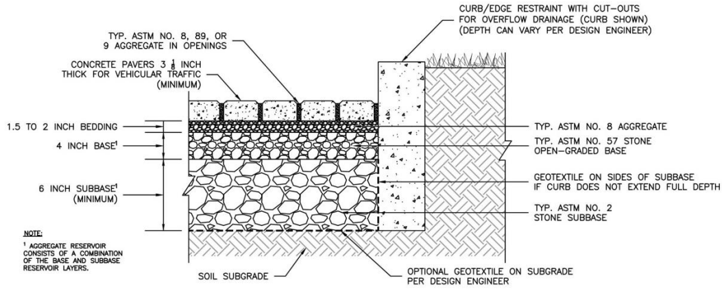
FULL INFILTRATION NTS
