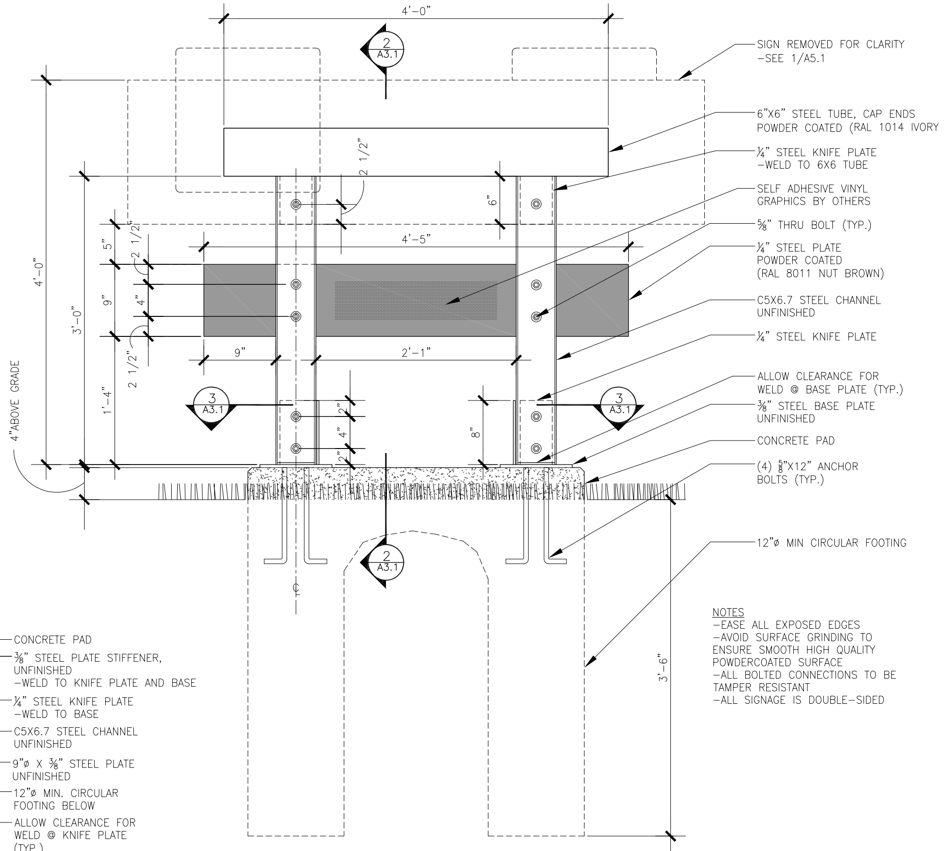
1 FRONT ELEVATION A3.1 1"=1'-0"
