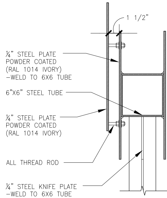
4 SIGN DETAIL A5.1 1 1/2"=1'-0"
