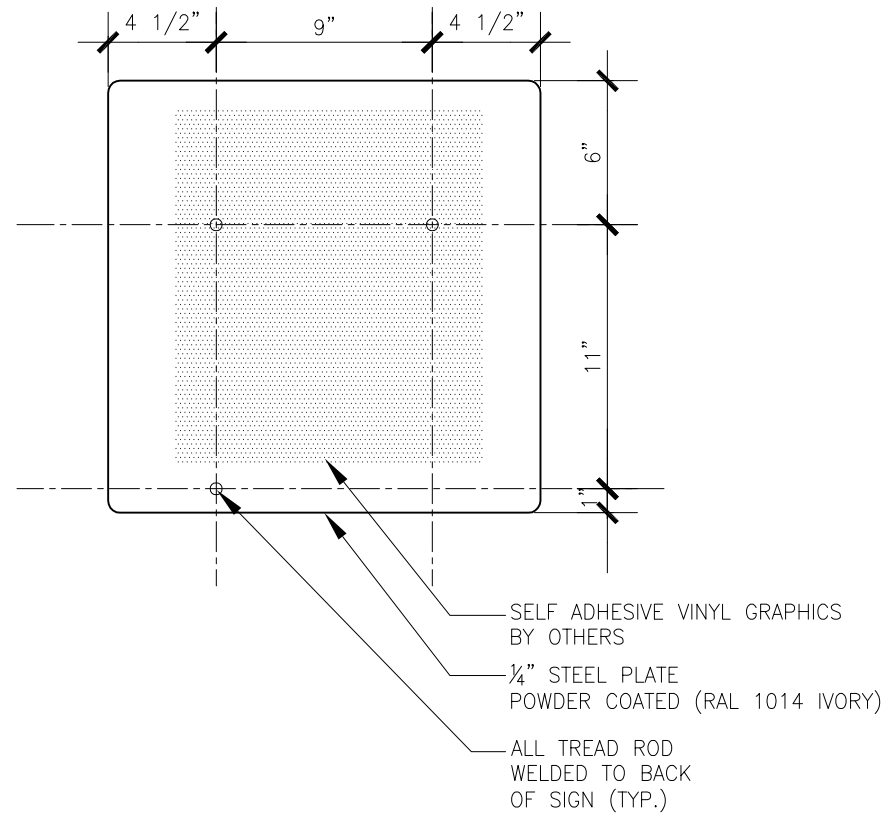
2 SIGN ELEVATION A5.1 1 1/2"=1'-0"
