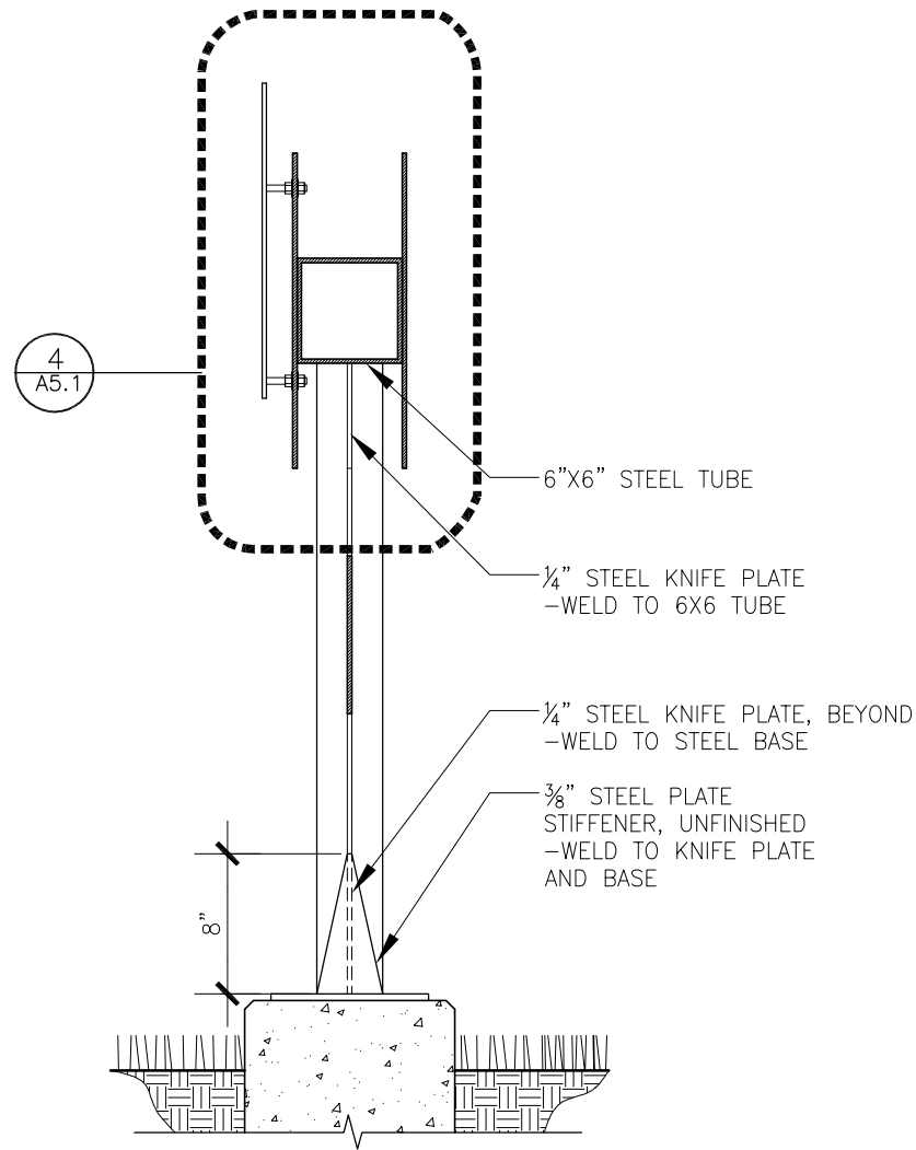
2 SECTION A3.1 1"=1'-0"
