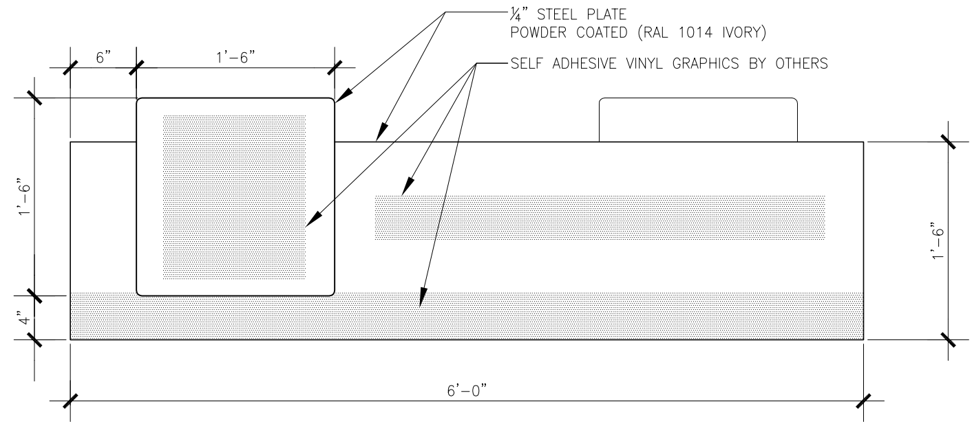
1 SIGN ELEVATION A5.1 1"=1'-0"
