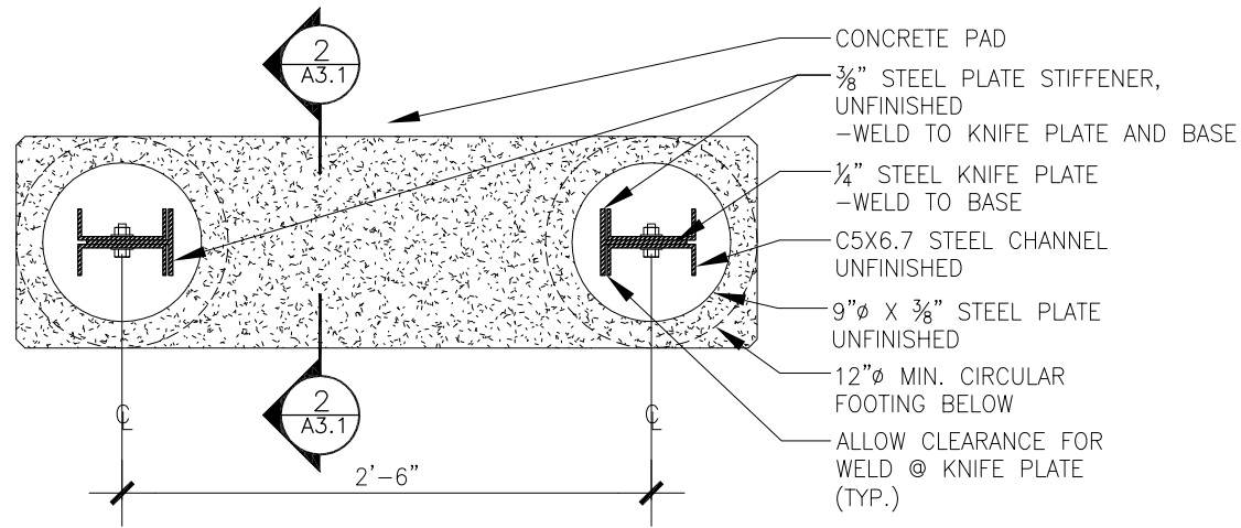
3 PLAN SECTION A3.1 1"=1'-0"
