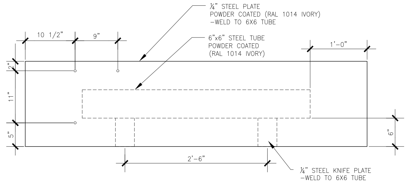
3 SIGN DETAIL A5.1 1"=1'-0"
